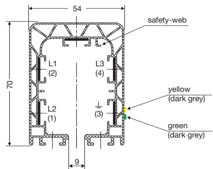
A - A KBH 5-conductors
