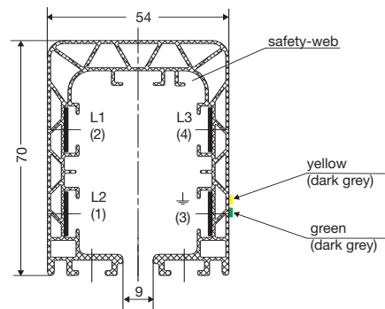
A - A KBH 4-conductors
